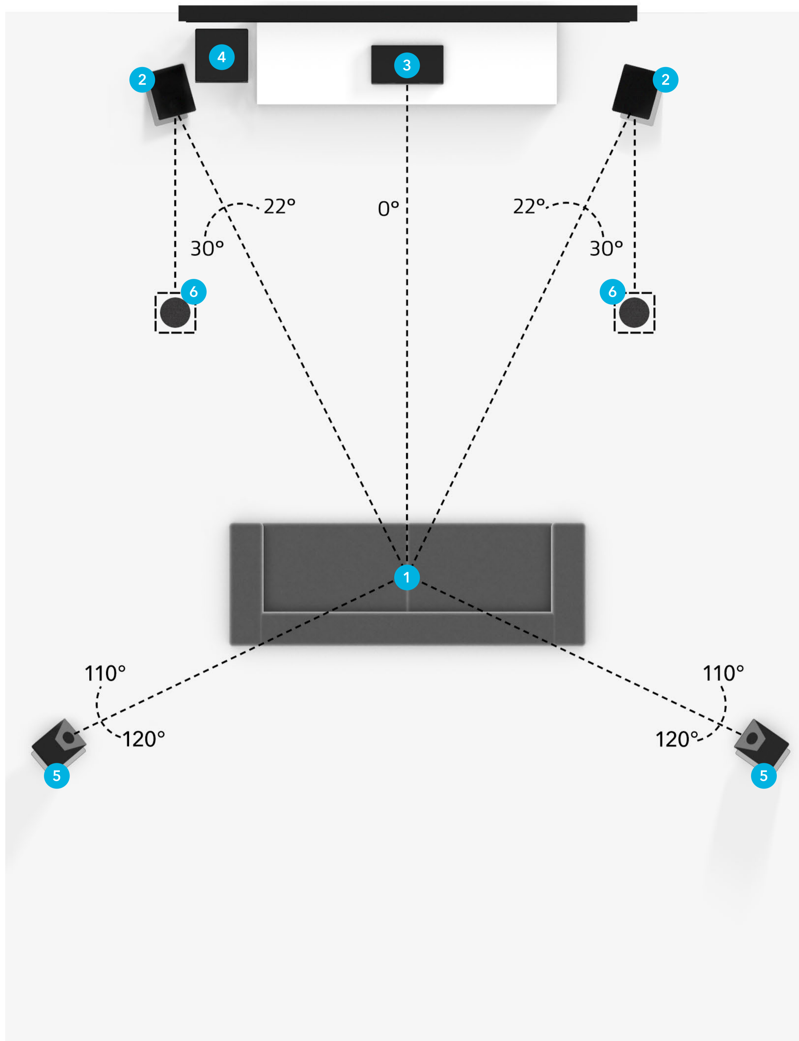
SPEAKER PLACEMENT FOR 5.1.4 SETUP
